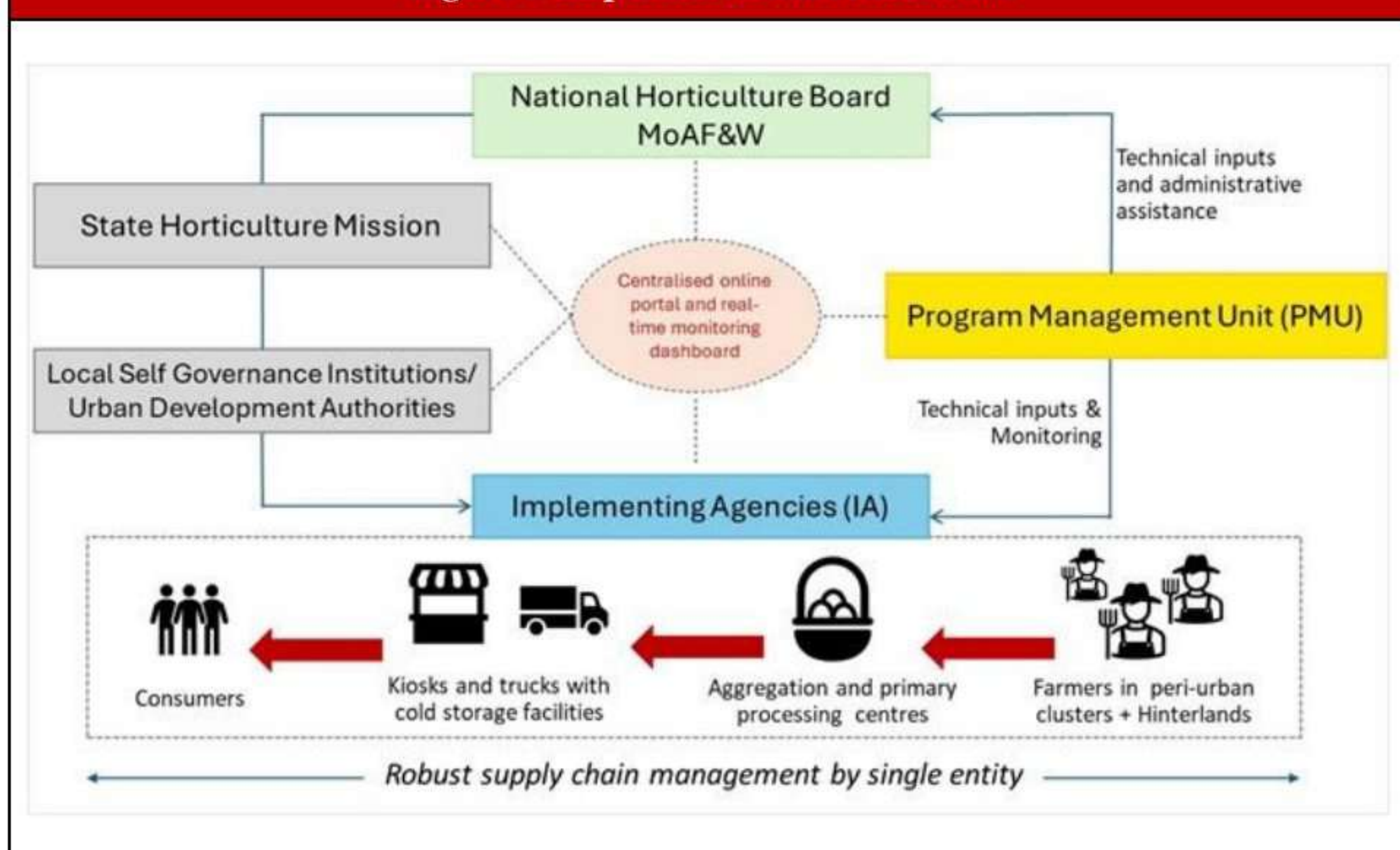
Figure 1: Implementation Framework
